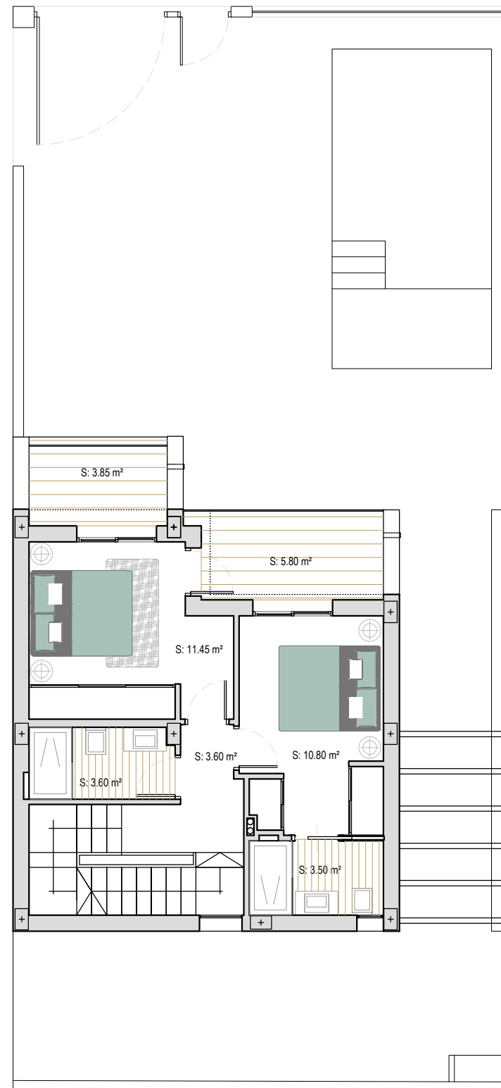
First floor
