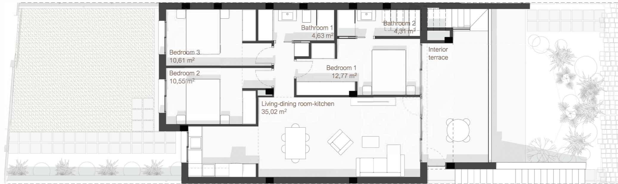
Penthouse
